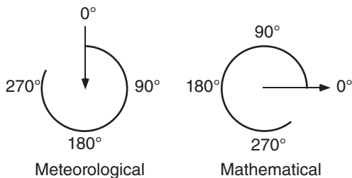
Figure 1.2 Comparison of meteorological and mathematical angle conventions.
