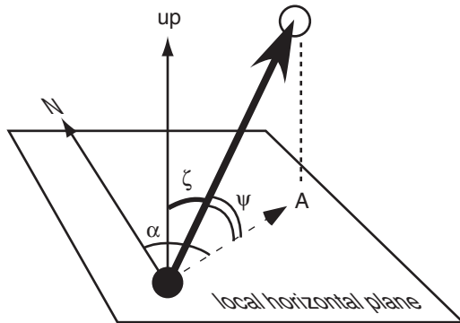
Figure 1.6 Elevation angle \Psi , zenith angle \zeta , and azimuth angle \alpha .
