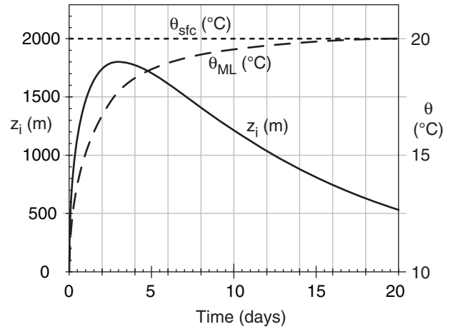
Figure 12.5 Genesis of a warm airmass after cold air comes to rest over a warmer surface. This is an example based on toy-model equations in the INFO Box. Airmass potential temperature is \theta_{ML} and depth is z_i . Imposed conditions for this case-study example are: large-scale divergence \beta = 10^{-6} \text{ s}^{-1} , potential temperature gradient in vertical \gamma_0 = 3.3 \text{ K km}^{-1} , initial near-surface air potential temperature \theta_{ML} = \theta_0 = 10^\circ\text{C} , and surface temperature \theta_{sfc} = 20^\circ\text{C} .
