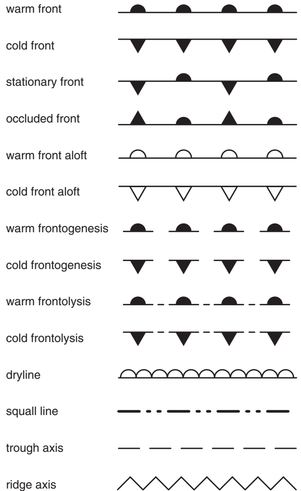
Figure 12.10 Glyphs for fronts, other airmass boundaries, and axes (copied from the Weather Reports and Map Analysis chapter). The suffix “genesis” implies a forming or intensifying front, while “lysis” implies a weakening or dying front. A stationary front is a frontal boundary that doesn’t move very much. Occluded fronts and drylines will be explained later.
