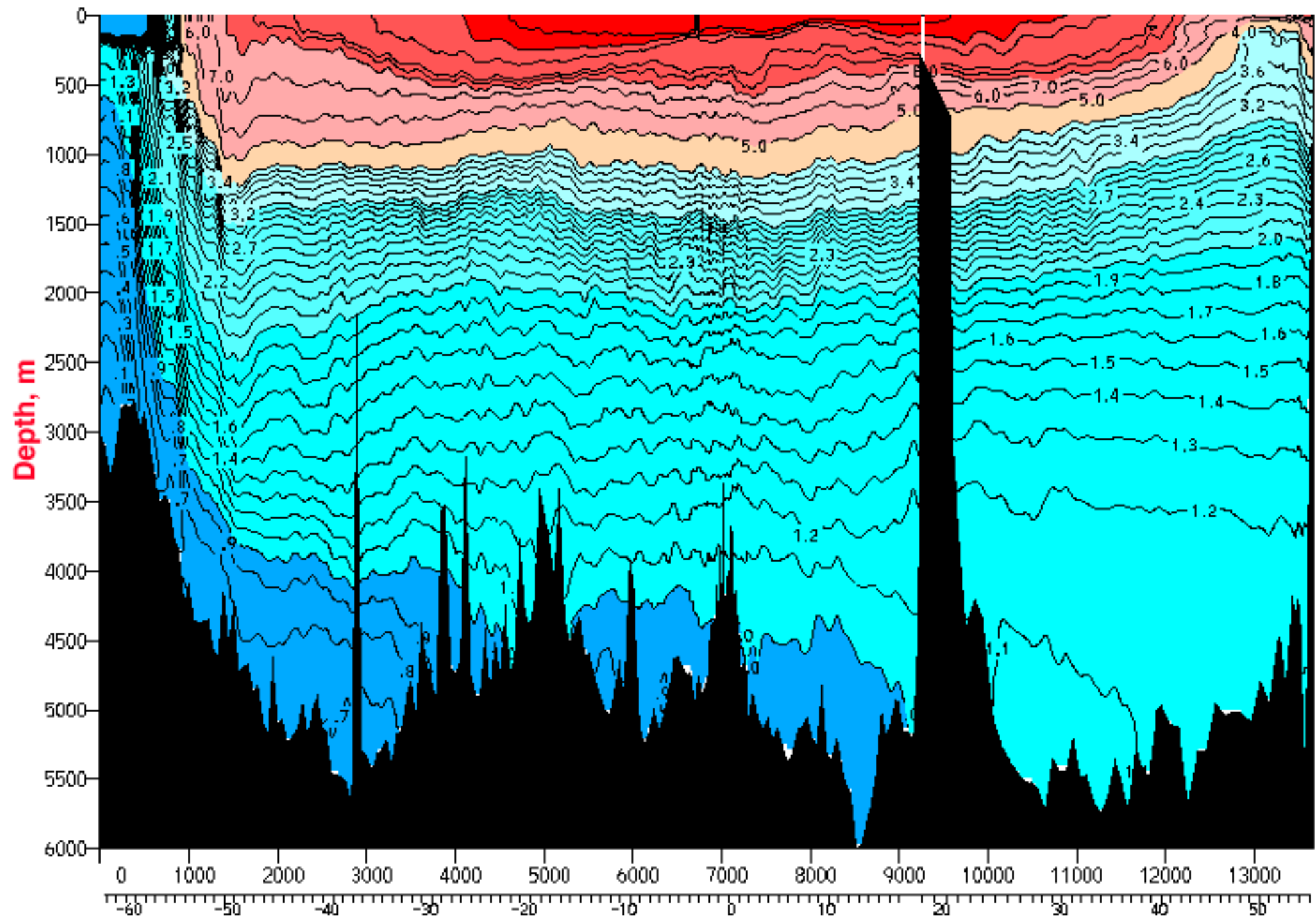
Pacific Ocean, Potential Temperature, Cross-Section Along 150 Deg. W, 1992
