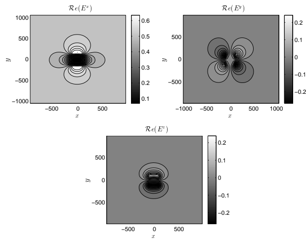
Figure 7: MT problem: contour plots of the computed solution \mathcal{R}e(\mathbf{E}) at the air-earth interface ( \mathbf{E} is scaled so that \mathbf{E}(x, y, z = 2000) = (1, 0, 0)^T ).
