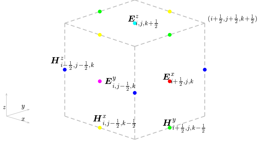
Figure 2: Staggered discretization of \mathbf{E} and \mathbf{H} in three dimensions.
