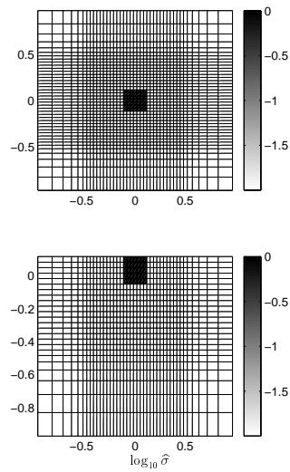
Figure 6: MT problem: a horizontal and a vertical cross-section of \log_{10} \sigma .
