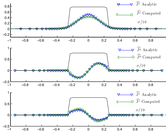
Figure 4: Synthetic problem: the real parts of computed current, \widehat{\mathbf{J}}_c , and the analytic current, \widehat{\mathbf{J}}_a , through a cross-section of the conductivity \widehat{\sigma} .
