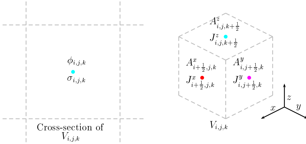
Figure 1: The cell V_{i,j,k} along with a cross-section. The cell V_{i,j,k} corresponds to a block of conductive material within which \sigma \approx \sigma_{i,j,k} .
