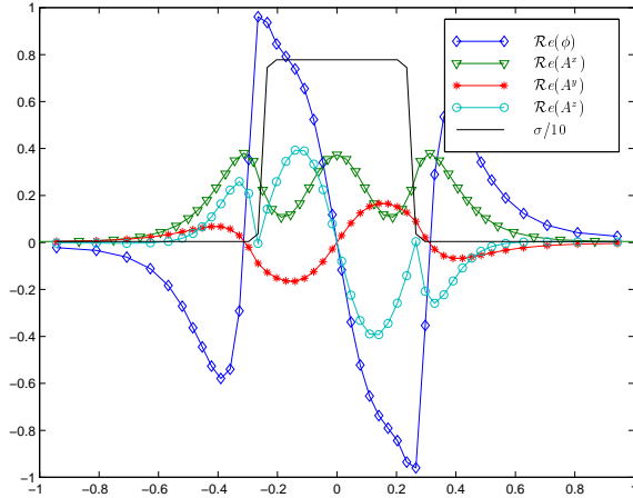
Figure 5: Synthetic problem: the real parts of computed solutions \mathbf{A} and \phi through a cross-section of conductivity \hat{\sigma} .
