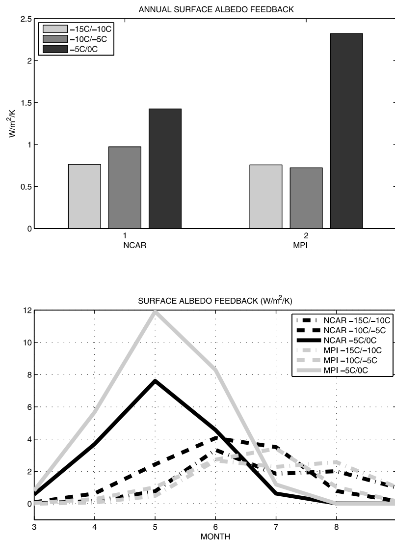
Figure 1. (top) Polar surface albedo feedback in three temperature eras. (bottom) Monthly contribution to polar surface albedo feedback for surface temperatures less than -5^\circ\text{C} (dashed) and between -5 and 0^\circ\text{C} (solid) for the NCAR CCSM3 (black) and MPI ECHAM5 (gray) models. All data have been boxcar filtered over a 5-year period.
