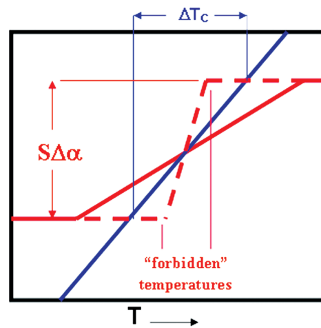
Plate 1. Schematic of the top-of-atmosphere absorbed shortwave radiation (red) and OLR (blue) as a function of surface temperature. The solid red absorbed shortwave profile is stable because the surface albedo transition occurs over a range of temperatures greater than \Delta T_c and so is less steeply sloped than the OLR curve. The dashed profile is unstable since the transition occurs over a smaller range of temperatures, leading to a region where increased shortwave absorption exceeds OLR cooling as temperature increases (a net positive feedback). Within this temperature range is a “forbidden” zone where no equilibrium is possible under changes in forcing. (Forcing changes can be thought of as moving the blue OLR curve left or right without changing its slope.)
