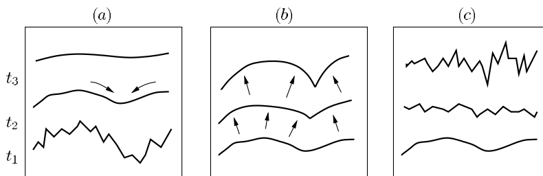
Figure 3 Three mechanisms of surface growth corresponding to the three terms of Equation 24. Diffusive smoothing is depicted in (a), growth normal to the surface in (b), and random growth in (c). Surfaces are shown for each mechanism at times t_1 , t_2 , and t_3 where t_1 < t_2 < t_3 . In (a), the arrows represent the flux of deposited material, and in (b) they indicate the direction of growth (for \lambda > 0 ).
