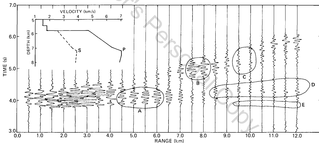
Figure 9. Velocity model and resultant horizontal component synthetic seismogram representing best fit to salient features (regions A-E) of Figure 8. Velocity model represents compressional and shear wave velocity structure of crust at Site 417. Figure from Stephen et al. (this volume).
