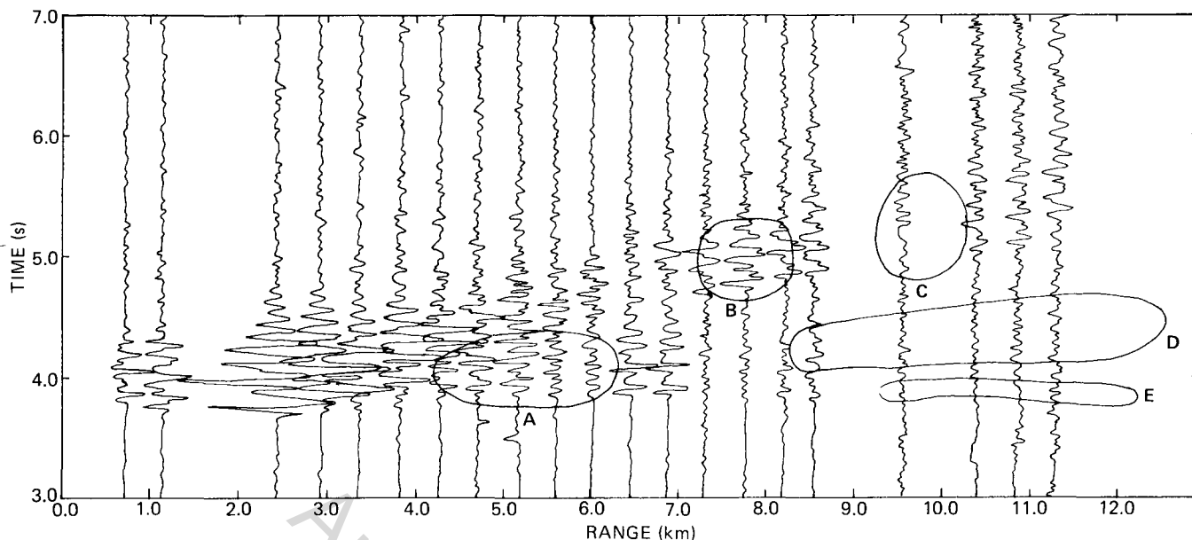
Figure 8. Observed north-south horizontal component data from south line of oblique seismic experiment at Site 417; geophone 228 meters into basement (6060 m below rig floor); amplitudes weighted by (\text{range}/7.0)^{2.9} for ranges greater than 7.0 km; time reduced to 6.0 km/s. Note signal character in regions A-E. Figure from Stephen et al. (this volume).
