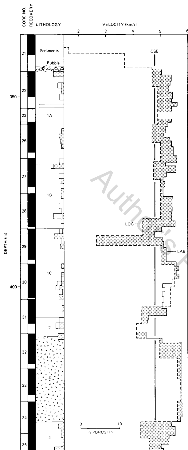
Figure 10. Comparison of compressional wave velocities obtained from logging, physical properties studies, and the oblique seismic experiment in Hole 417D (see text). Discrepancy between laboratory and logging data (stippled area) is a measure of formation porosity due to open cracks. Units 1, 2, and 4 are composed of pillow basalts, while Unit 3 (hachured) is composed of massive basalt; insets in lithology column represent abundance of limestone (plain) and smectite (light gray) on a scale of 0 per cent to 50 per cent.
