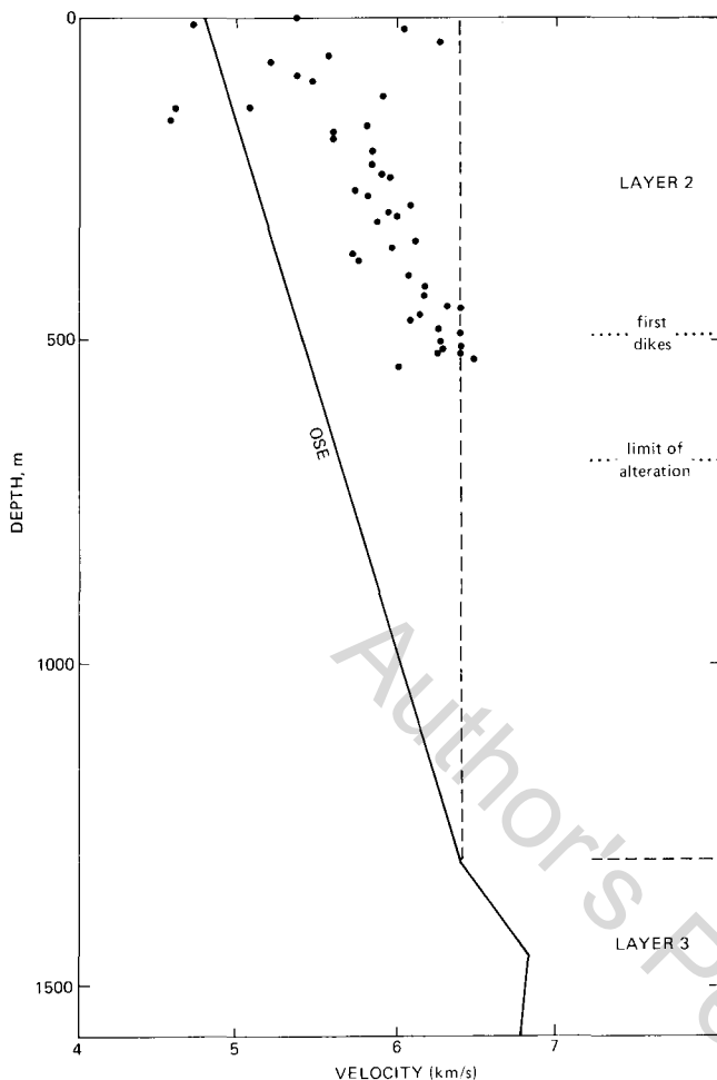
Figure 11. Comparison of laboratory velocities of samples from Hole 418A (Christensen et al. , this volume) and the results of the oblique seismic experiment in Hole 417D (Stephen et al. , this volume). Laboratory velocities measured at an effective confining pressure of 0.1 kbar. Vertical dashed line represents velocity of fresh basalt at 1.0 kbar.
