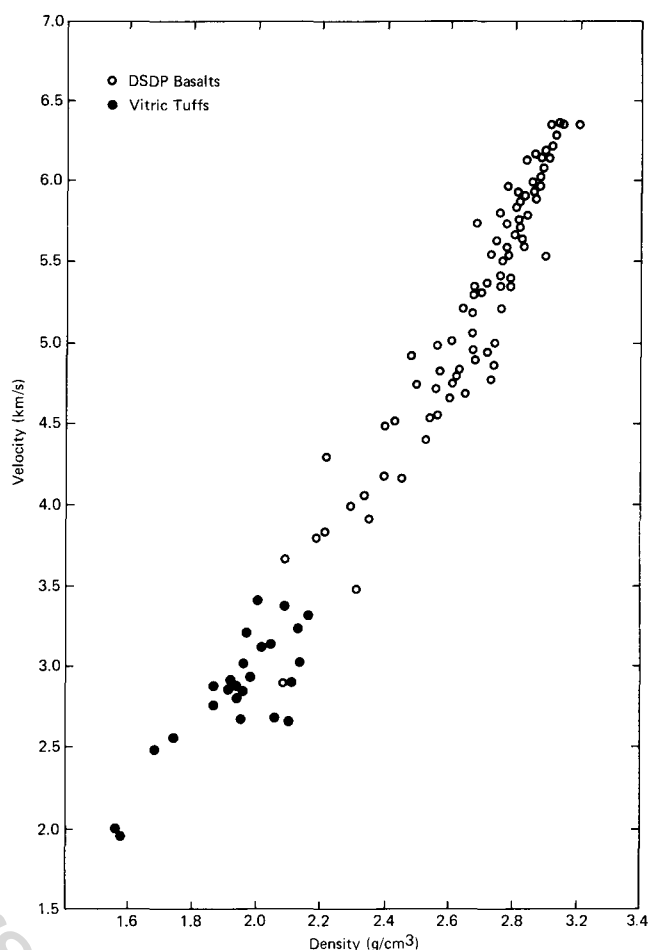
Figure 2. Compressional-wave velocity measured at 0.2 kbar versus density for Leg 59 sediments and DSDP basalts. (Sources of the basalt data are reported in text.)
