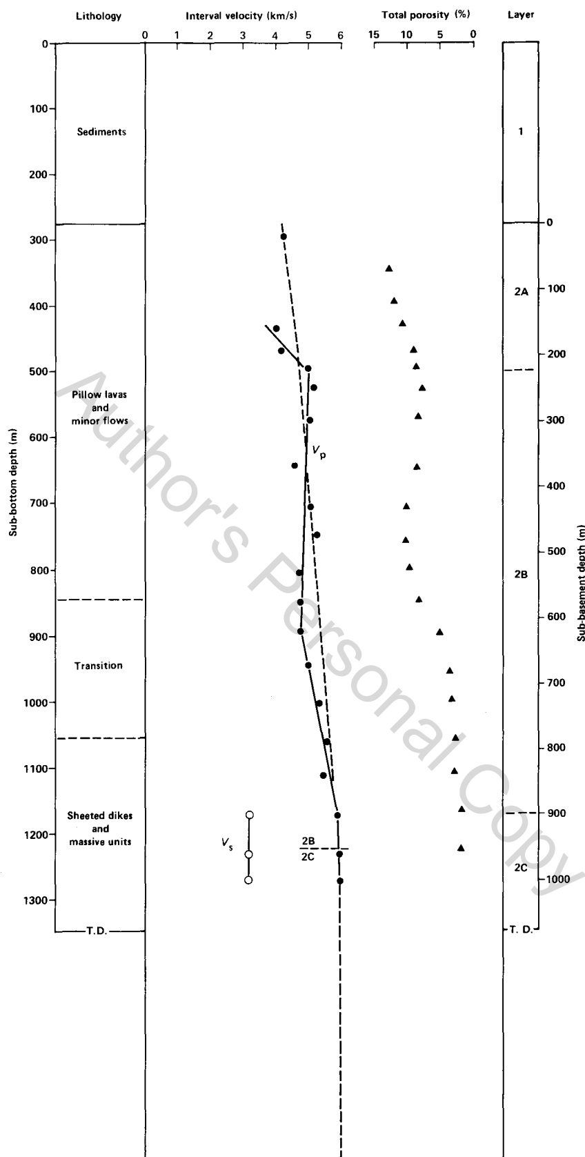
Figure 8. Summary of interval velocities and formation porosity versus depth and lithology in Hole 504B. Also shown are subdivisions defined using the velocity criteria of Houtz and Ewing (1976) for Layers 2A, 2B, and 2C and the velocity structure (dashed line) determined by means of the oblique seismic experiment at Site 504 (Stephen and Harding, 1983).
