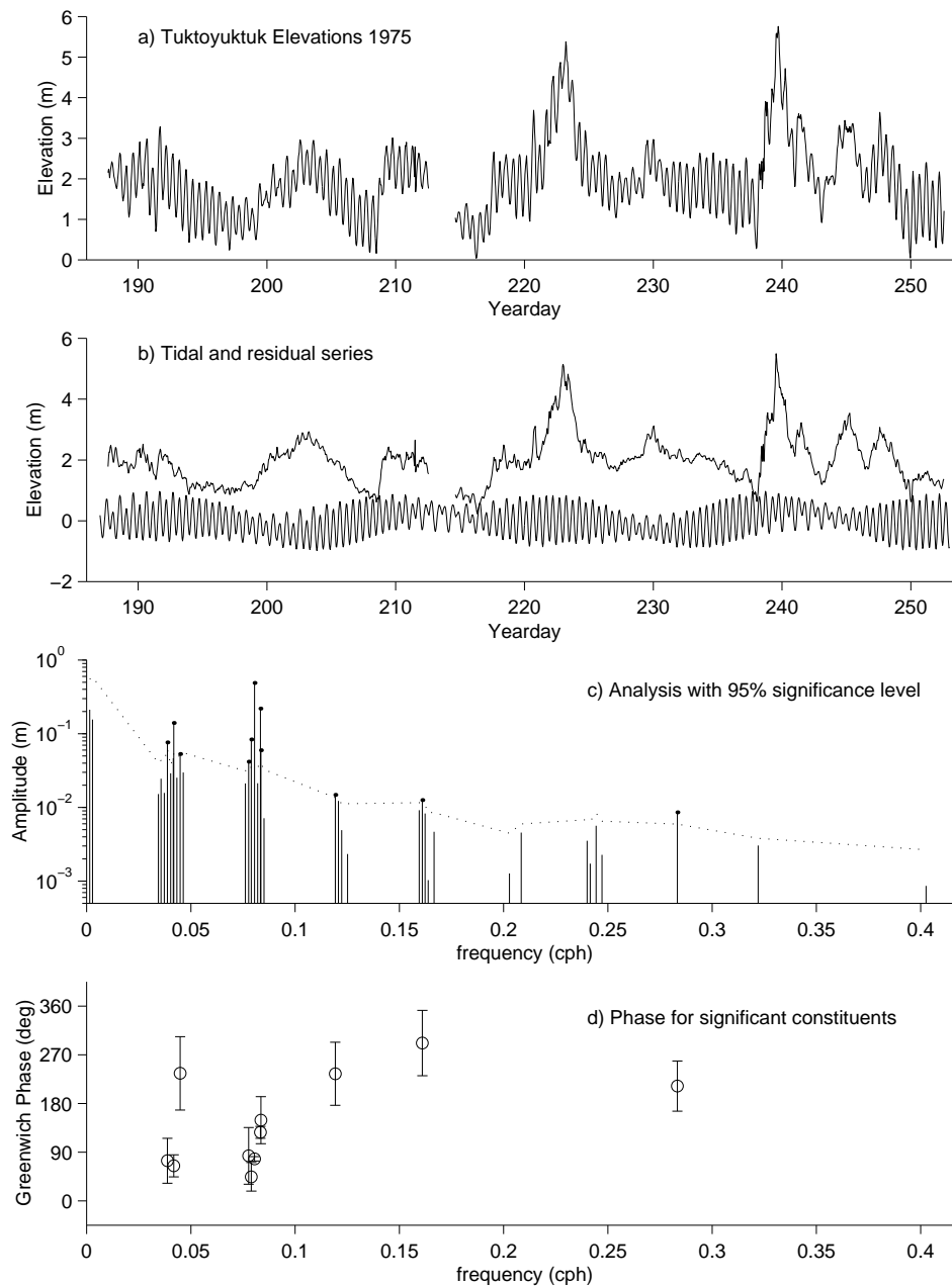
Fig. 1. Tuktoyuktuk analysis example. (a) Raw time series. (b) Upper curve is residual time series after removal of tidal signal. Lower curve is a synthesized tidal series using significant constituents. (c) Amplitude of all analyzed components with 95% significance level. Note frequency dependence. Significant constituents are marked with a solid circle. (d) The phase of significant constituents with a 95% confidence interval.
