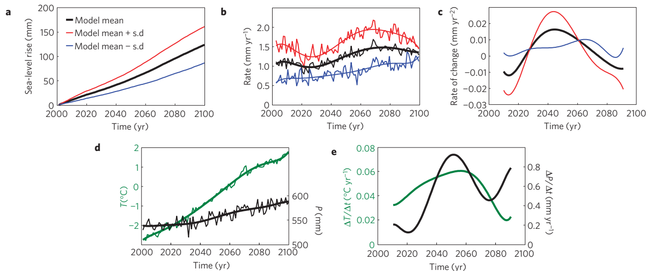
Figure 2 | Model projections for 2001–2100. a–e, Contribution of glacier wastage to sea-level rise, expressed in SLE ( a ), rate of sea-level rise including polynomial fit ( b ) and its rate of change ( c ), multi-model mean of annual temperature and precipitation projections (Fig. 1) including polynomial fit ( d ), and their annual rates of change ( e ). The black line in a–c denotes the model mean from 10 GCMs, red is the model mean + standard deviation and blue is the model mean – standard deviation. As the polynomial fit is not well constrained at the edges, the results for the first and last ten years in c and e are not shown.
